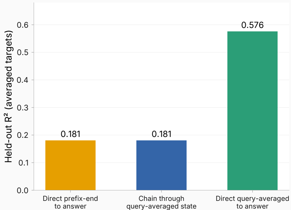
Chain test: deficit not linearly recoverable
