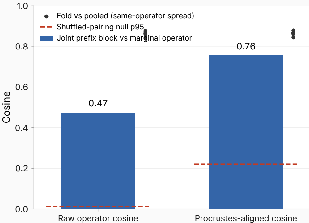
Joint vs marginal prefix operator (L14)
