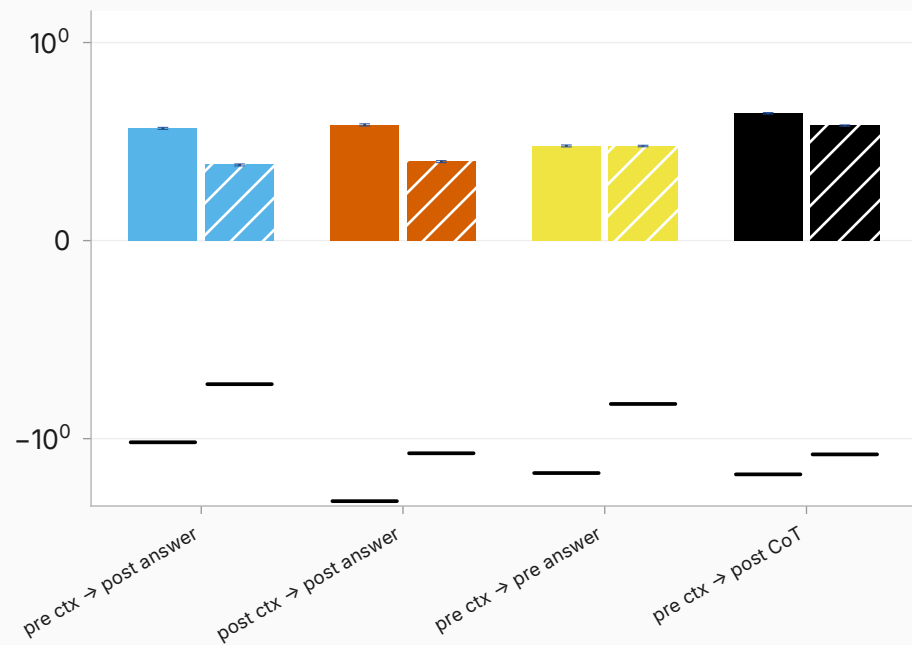
arm 2 — R1-Distill-Qwen-7B (pre: Qwen2.5-Math-7B)
