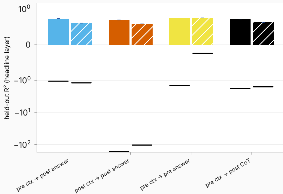
arm 1 — OpenThinker3-7B (pre: Qwen2.5-7B-Instruct)
