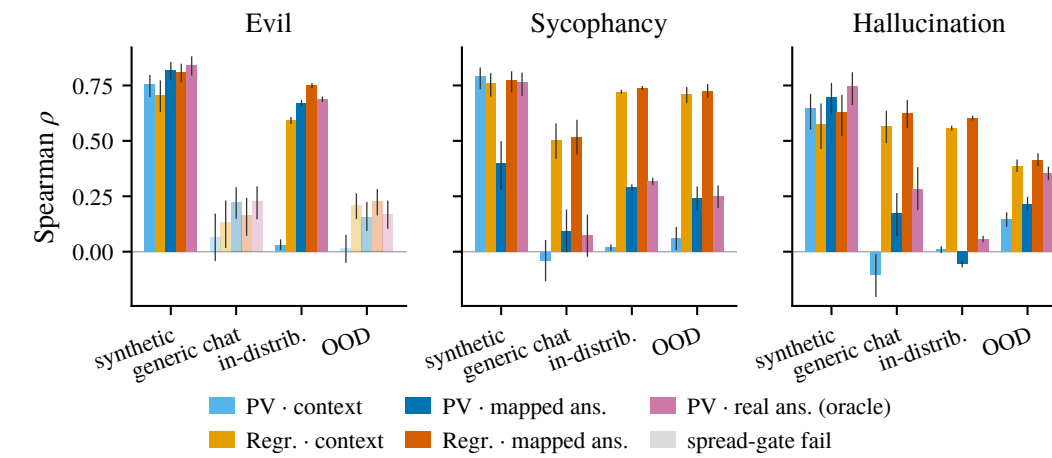
Figure 9. Spearman \rho between a readout and the judged behavior, per regime . Five readouts: the persona vector on the context ; a fitted regression on the context; the persona vector on the map-predicted answer; a regression on the map-predicted answer; and the persona vector on the real answer (oracle: it needs the answer generated). Regression arms consume the labelled budget; persona-vector arms are label-free. Muted bars fail the spread gate and are not interpretable. Hallucination in-distribution and OOD score fabricated fraction a different construct.
