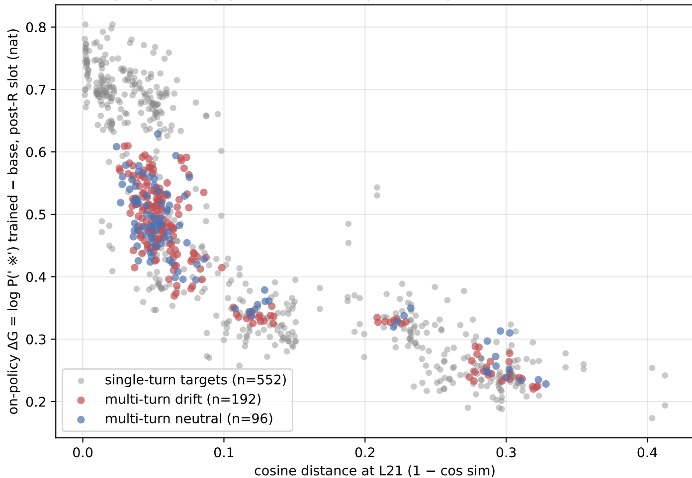
merged geometry-predicts-transfer panel: single-turn + multi-turn targets
