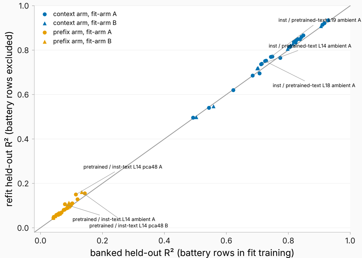
All 64 refit units (4 cells x layers x arms x bases; max |\Delta| 0.036)
