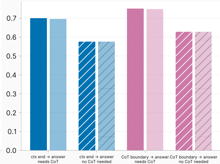
arm 3 — Qwen3-8B think on/off (different geometry)
