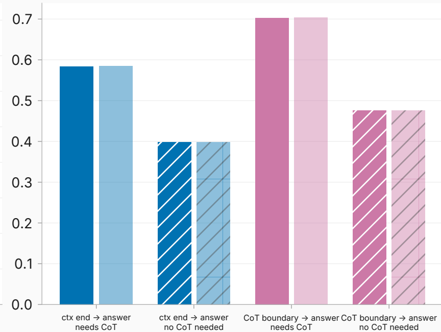
arm 2 — R1-Distill-Qwen-7B (pre: Qwen2.5-Math-7B)
