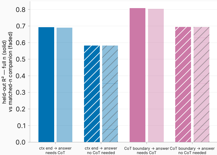
arm 1 — OpenThinker3-7B (pre: Qwen2.5-7B-Instruct)
