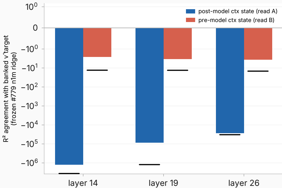
frozen n1m read — GSM8K test (arm 1)
