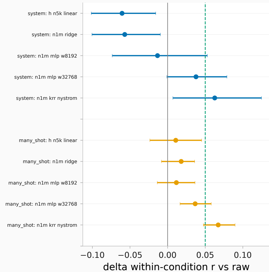
hallucination
