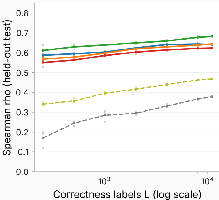
Short-answer QA (TriviaQA)
