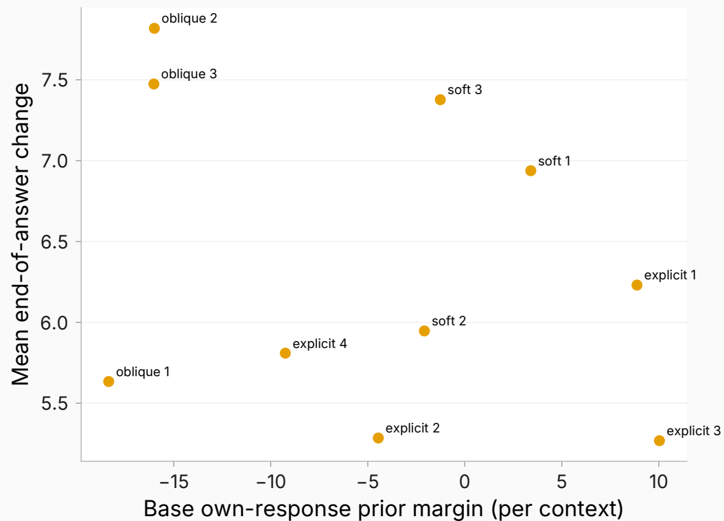
Prior gradient among never-clamped contexts ( \rho = -0.24 , n = 10 )
