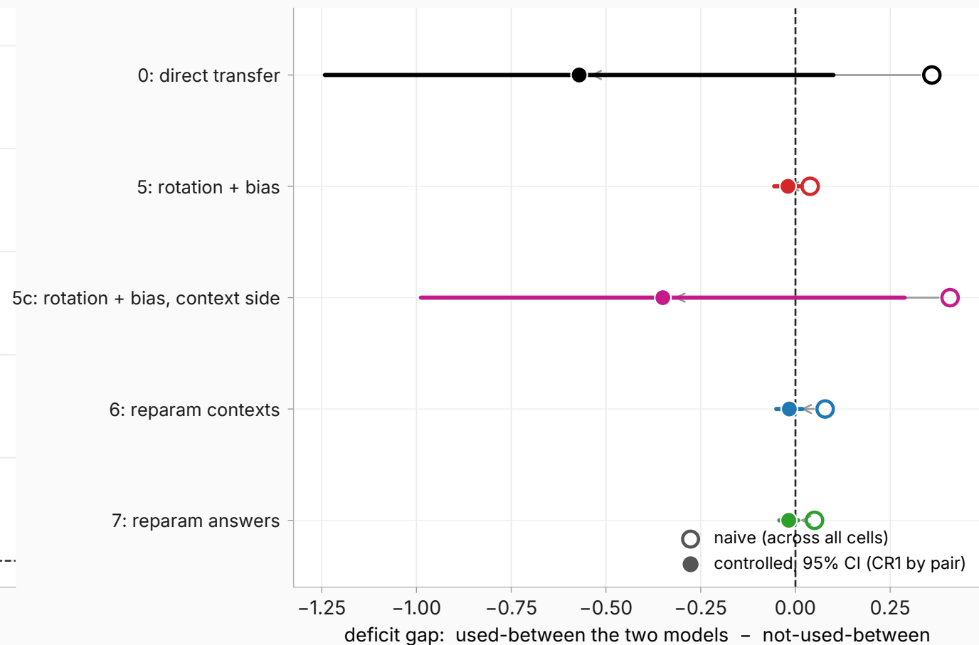
Naive gap → gap with pair and corpus effects removed
