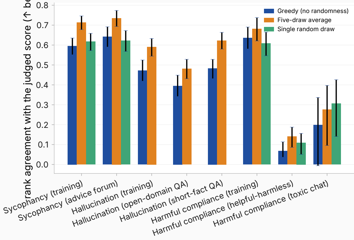
Raw agreement: the five-draw-average score ranks best
