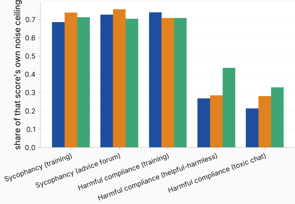
After the noise-ceiling correction it mostly closes
