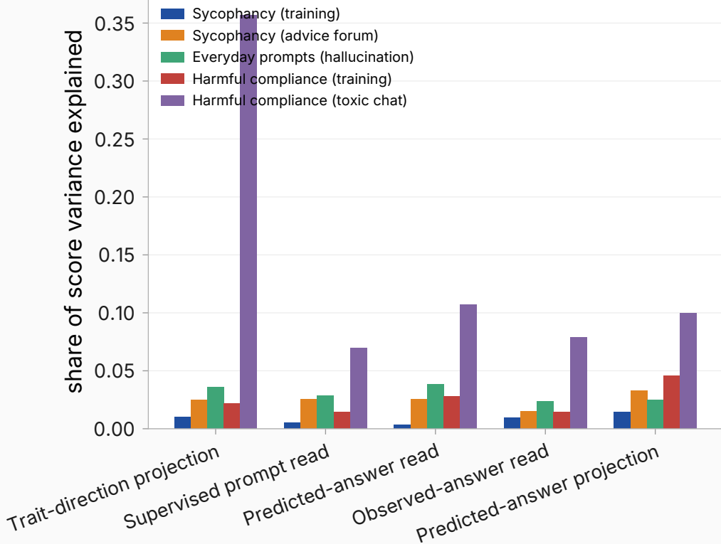
Explained share is small outside the smallest cell
