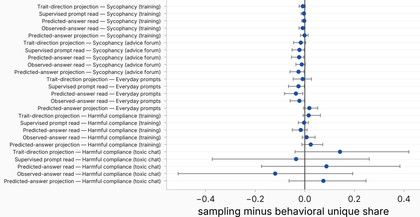
Per-arm contrasts: intervals straddle zero
