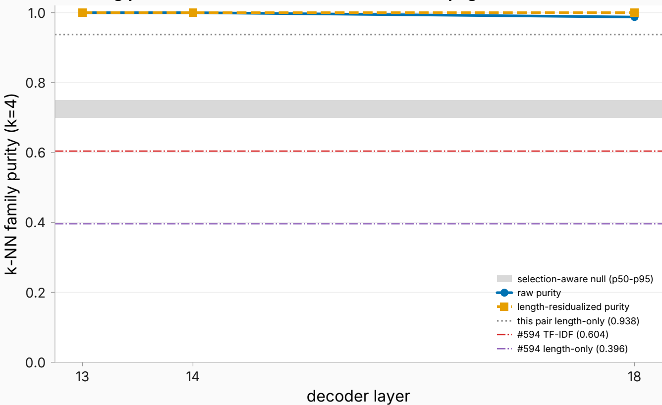
Winning pair kmeans10_c01 vs kmeans10_c08 (p_global=0.0010)
