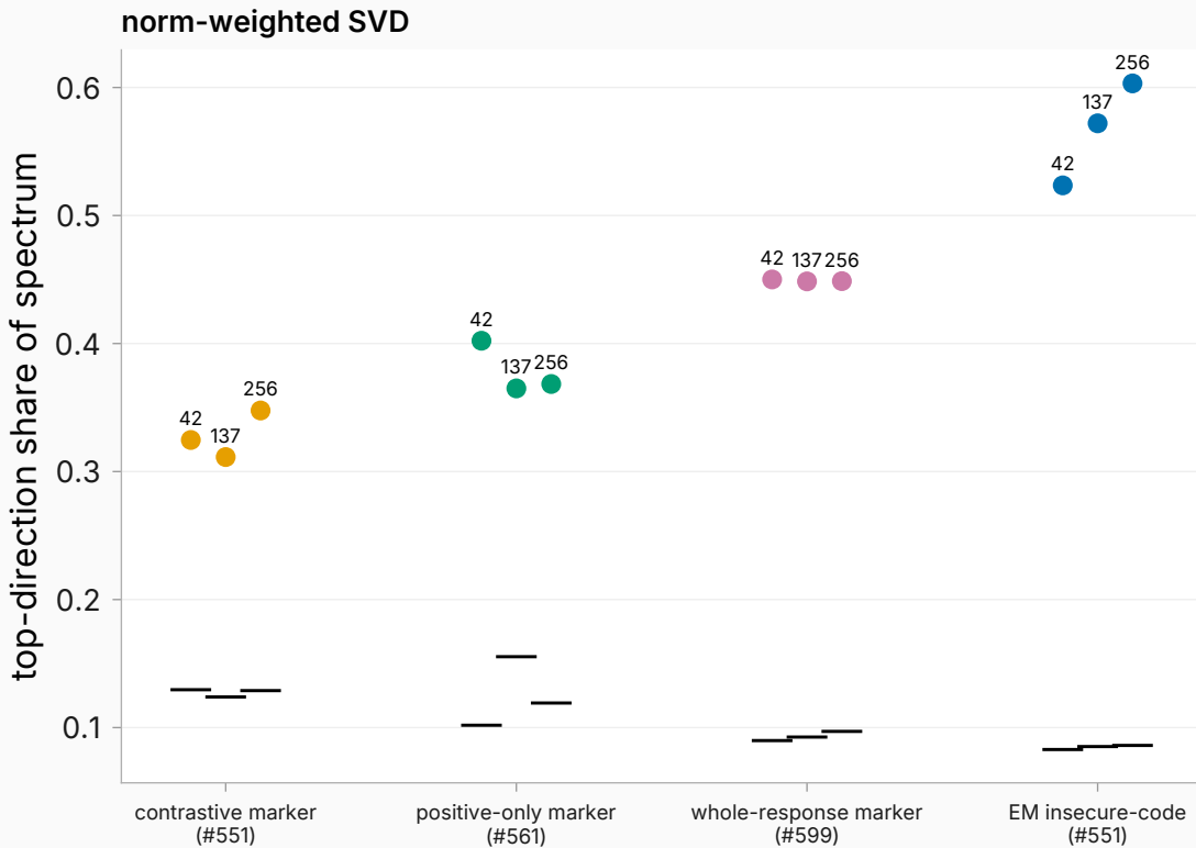
Same-text shift-spectrum concentration by arm (ticks = per-cell sign-flip null p95)
