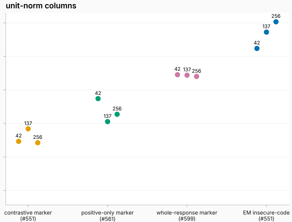
Same-text shift-spectrum concentration by arm (ticks = per-cell sign-flip null p95)
