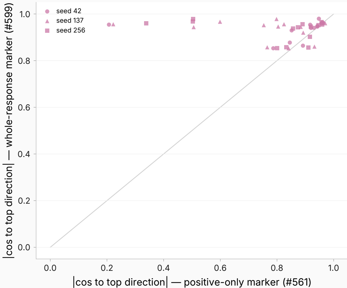
Per-persona alignment: whole-response vs positive-only (same-text)
