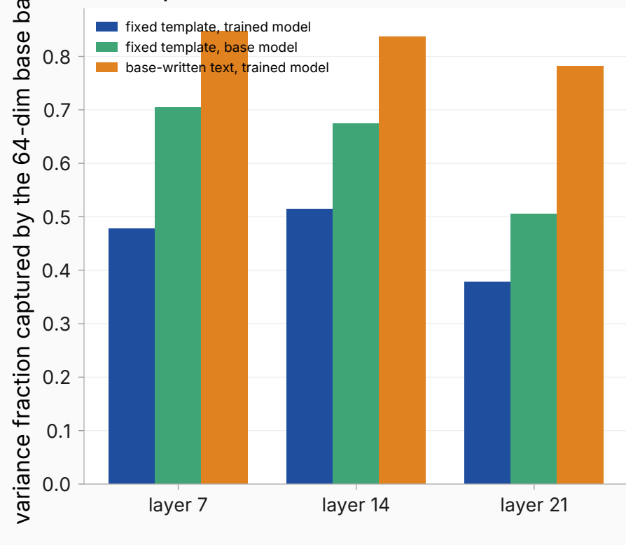
answer-profile variance inside the fit basis
