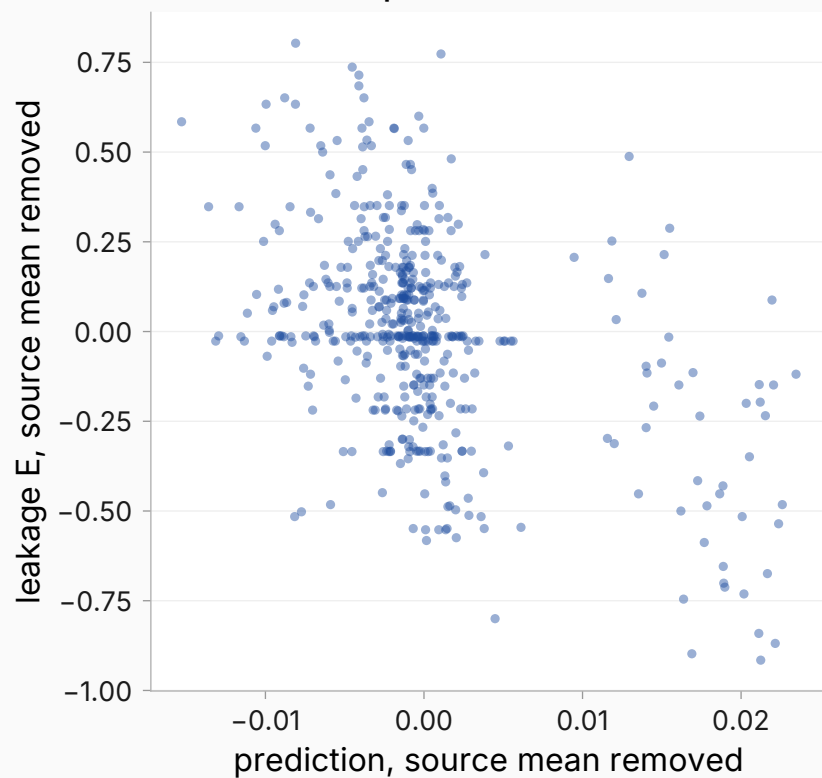
within sources: Spearman -0.39 (n=480)
