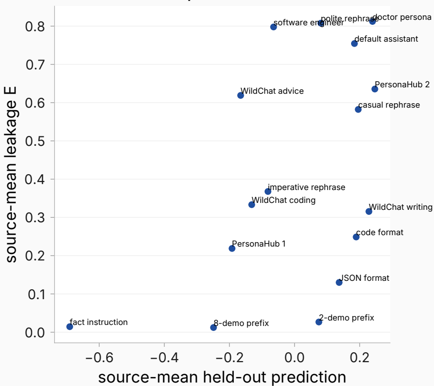
between sources: Spearman +0.51 (n=16)
