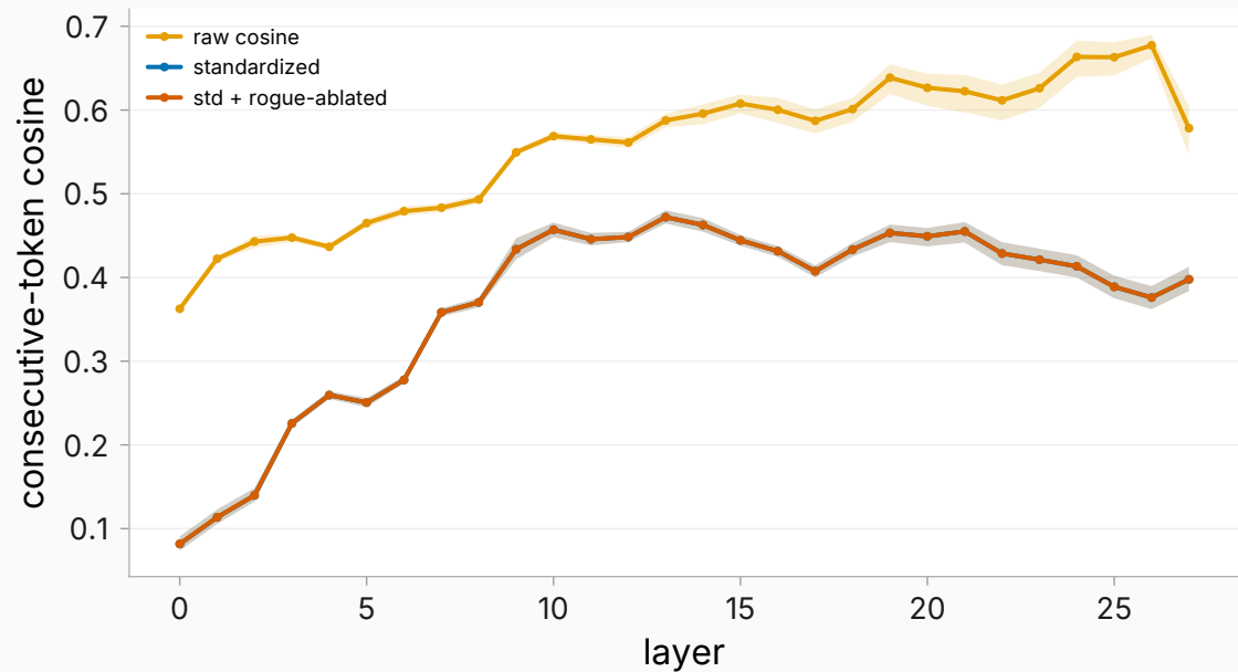
natural_stories
