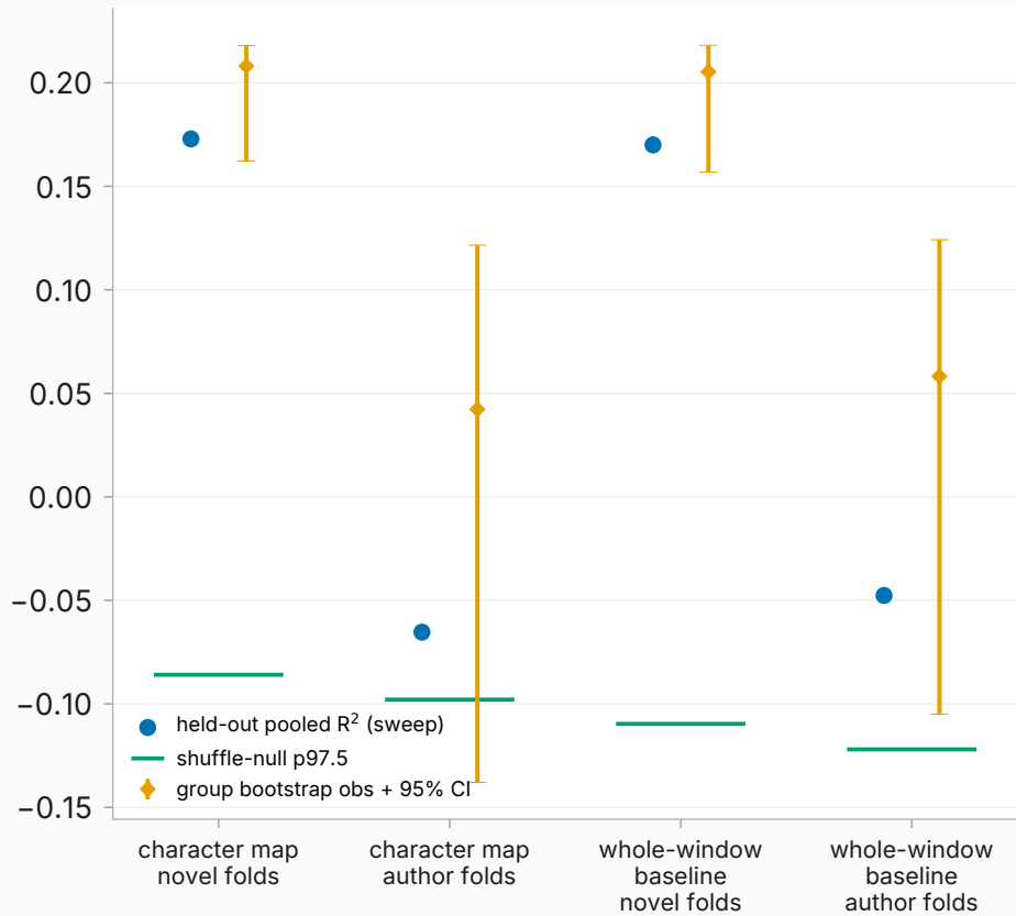
held-out pooled R^2 (layer 19)
