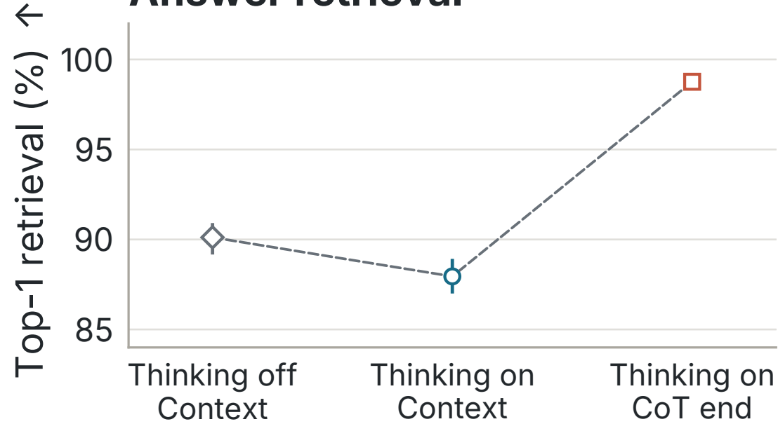
B · QWEN3-8B · NEEDS REASONING Answer retrieval
