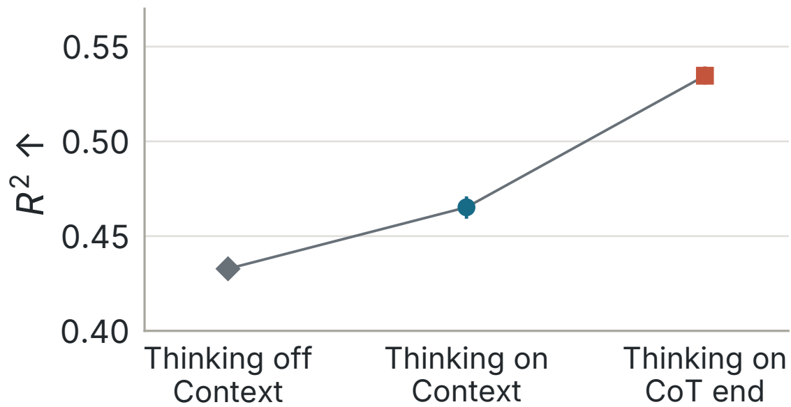
A · QWEN3-8B · NEEDS REASONING Answer predictability
