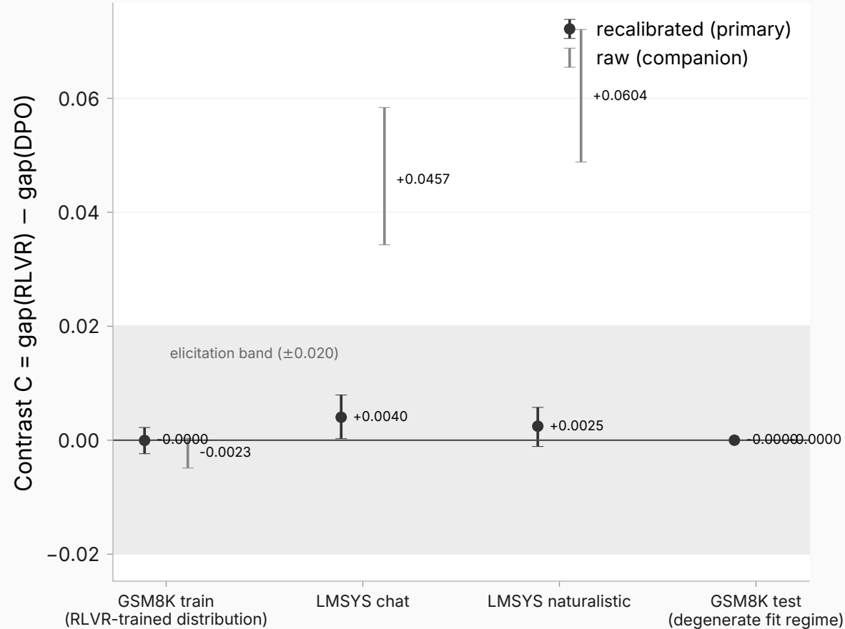
RLVR-specific contrast, 1000-draw paired bootstrap 95% CI
