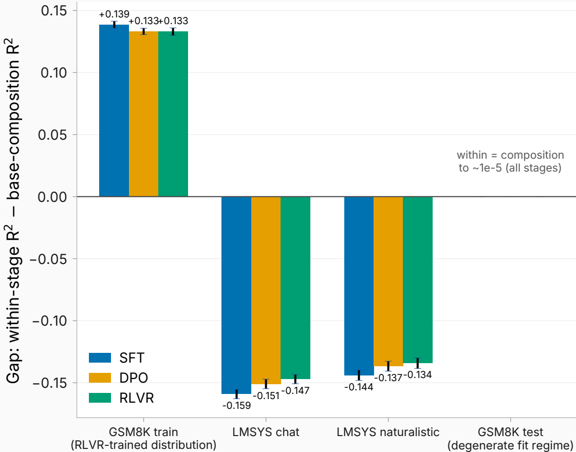
Gap per post-training stage (recalibrated scale, layer 30)
