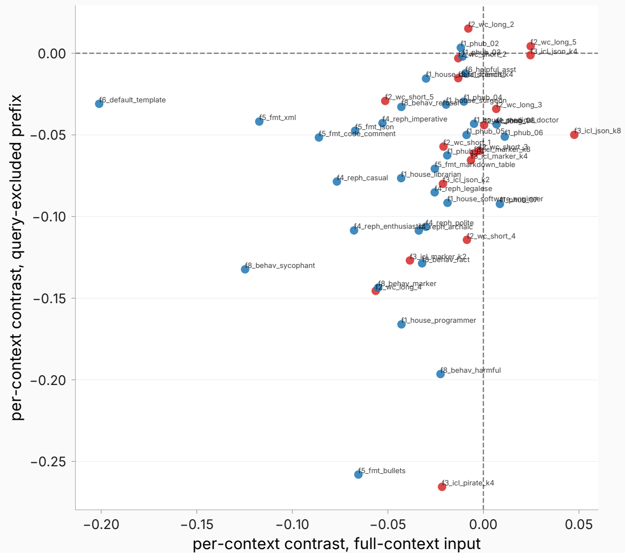
Query-averaged (layers 19/2)
