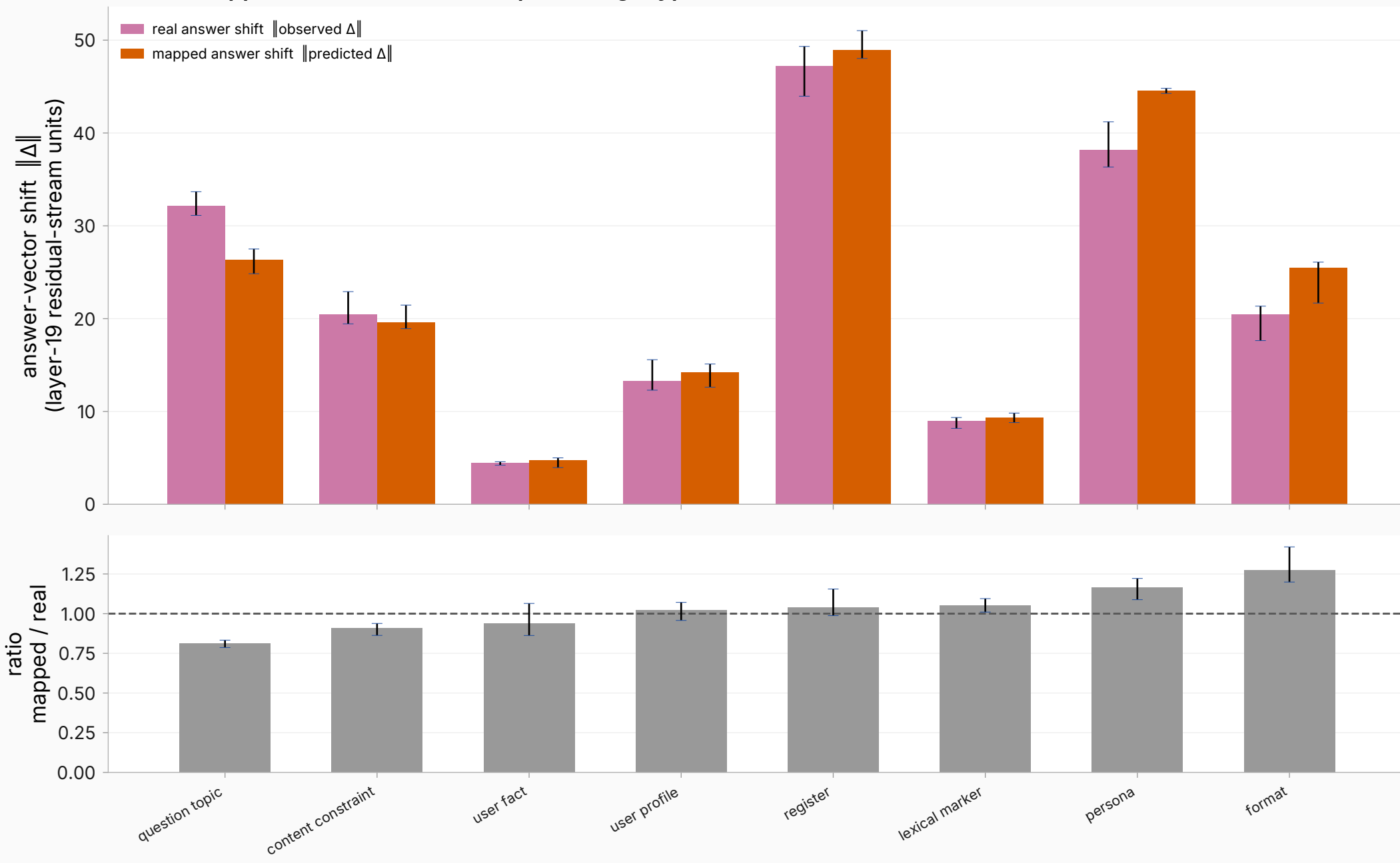
Real vs mapped answer-vector shift per change type (#2564)
