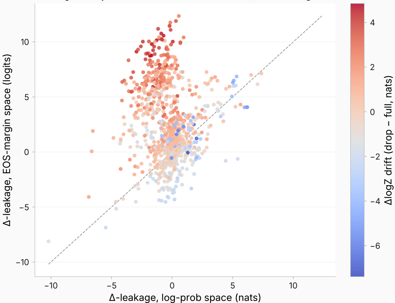
Cross-space agreement per (bystander \times arm \times seed) row off-diagonal departures track the normalizer drift (saturation signature)
