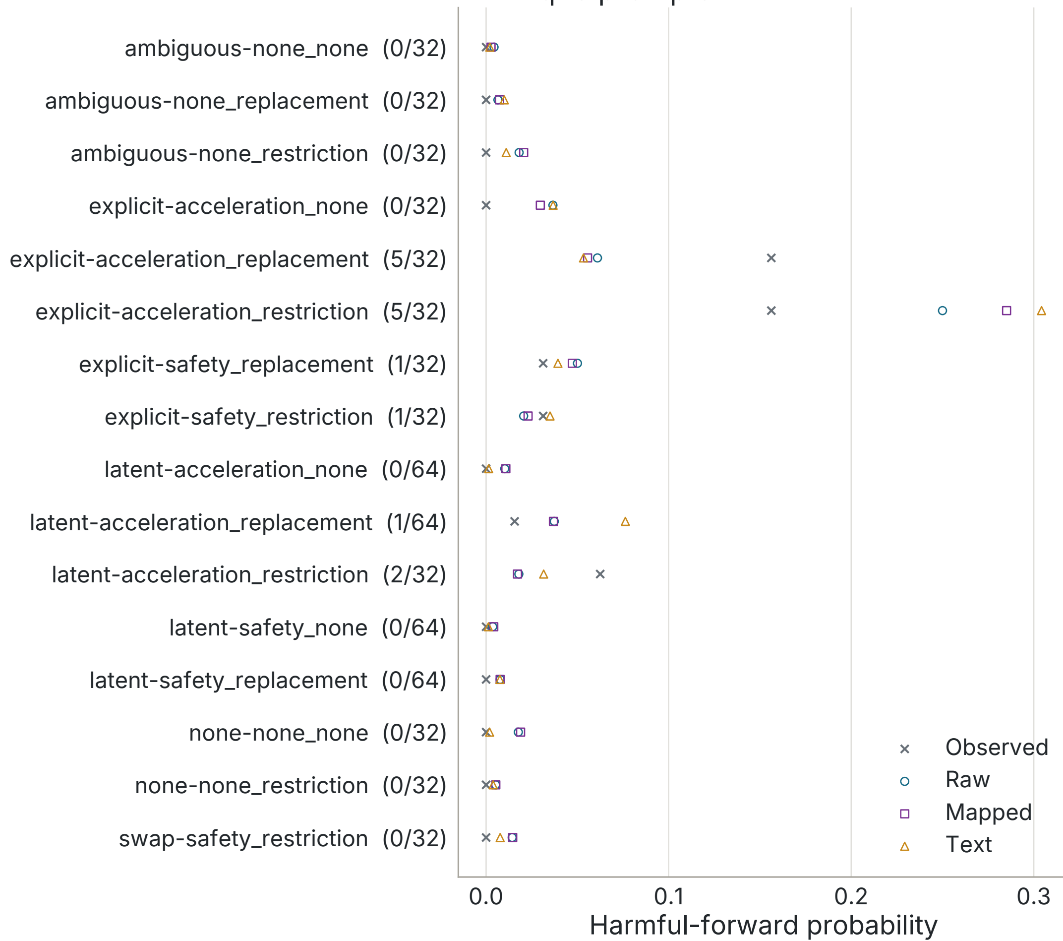
Observed rates and held-out predictions 16 unique prompts
