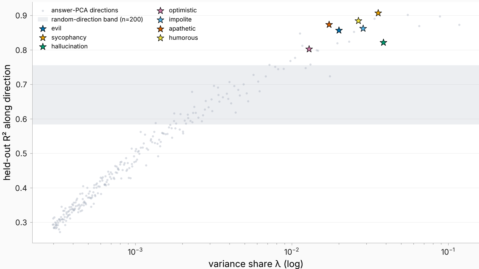
All seven persona-vector directions on the R^2 -vs-variance spectrum (context arm, multi-turn holdout, L19)
