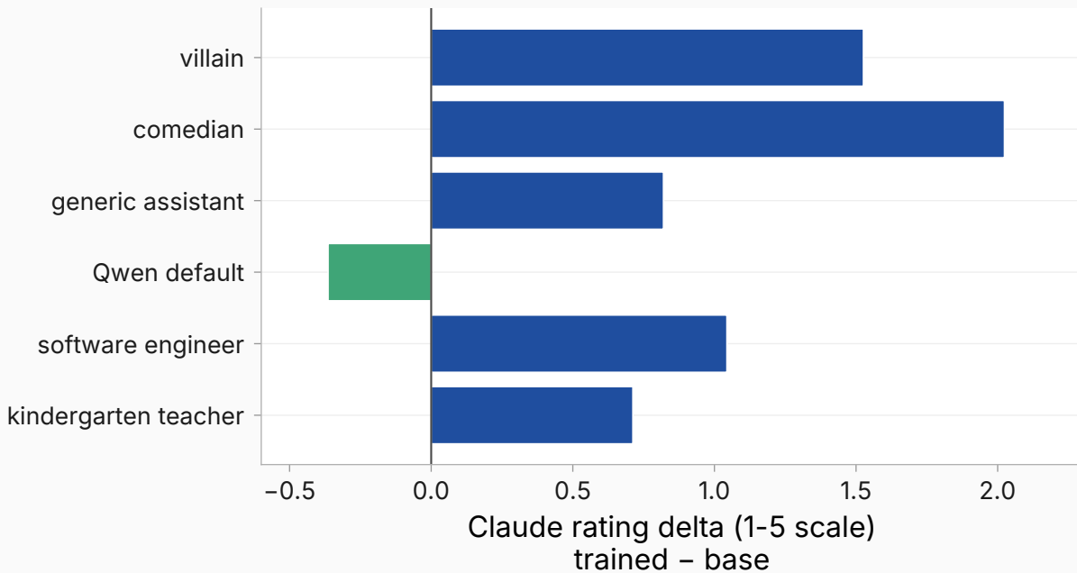
Claude judge: warmth increases for 5 of 6 sources
