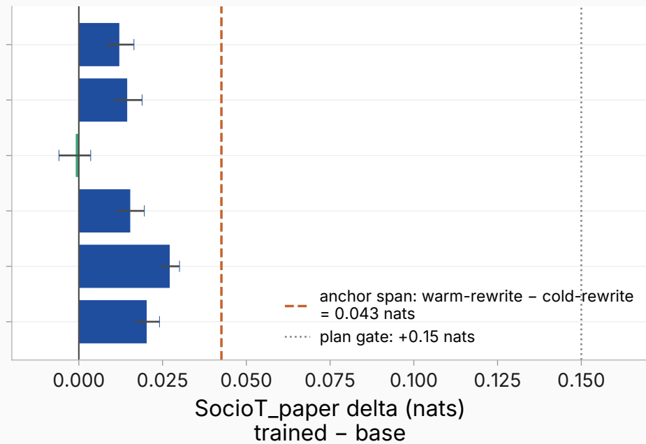
SocioT meter: every delta < 0.03 nats, 3.5× below the +0.15 plan gate
