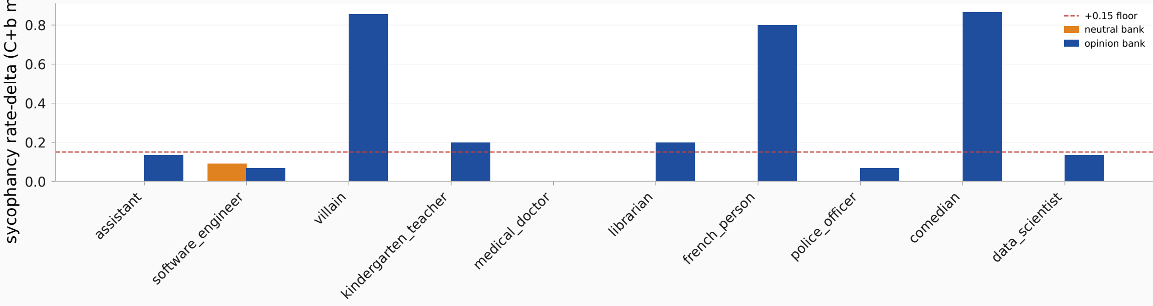
Sycophancy rate-delta: neutral vs opinion question bank
