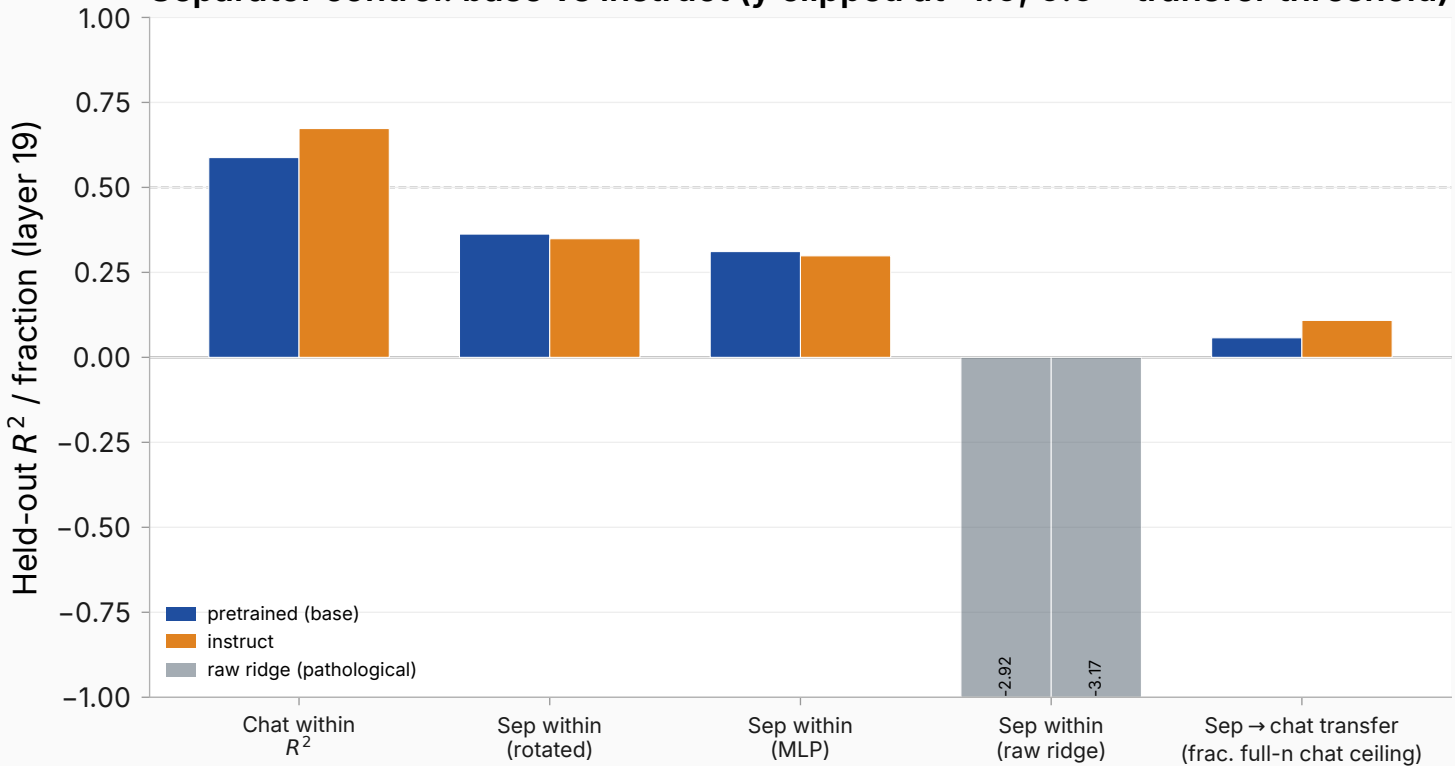
Separator control: base vs instruct (y clipped at -1.0; 0.5 = transfer threshold)
