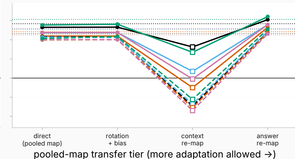
Qwen2.5-7B-Instruct
