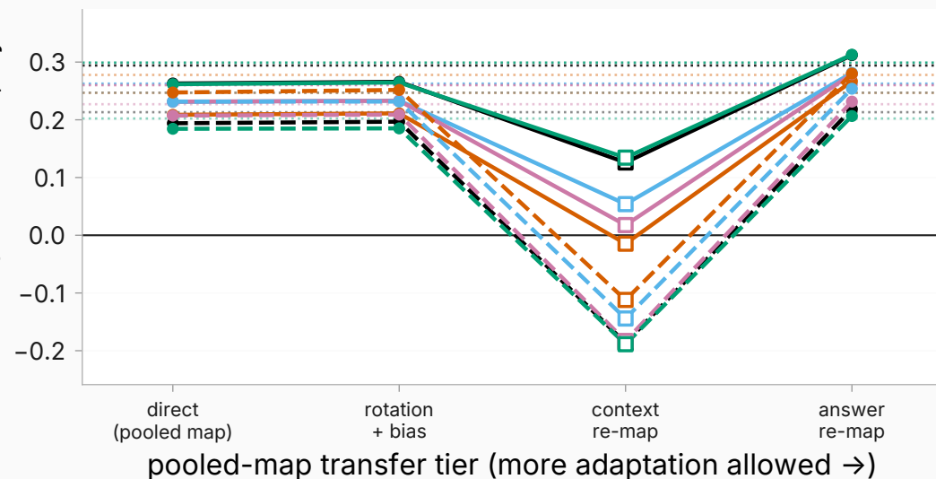
Qwen2.5-7B (base)
