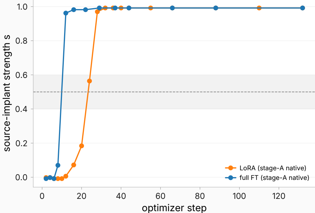
refusal: stage-A install trajectory
