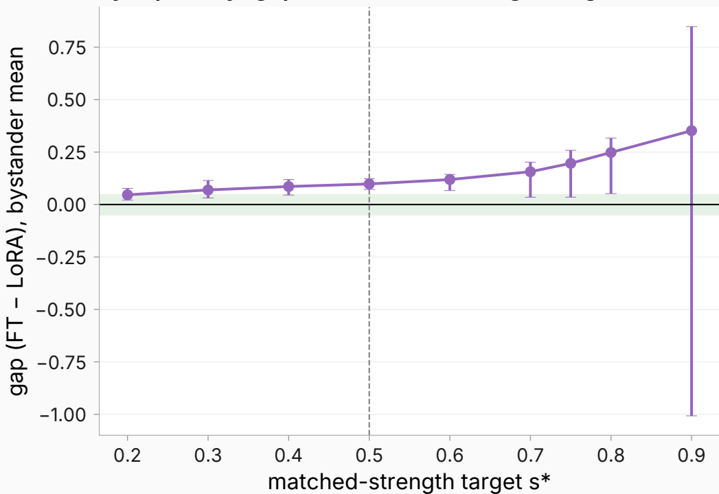
sycophancy: gap vs matched-strength target (x = out of range)
