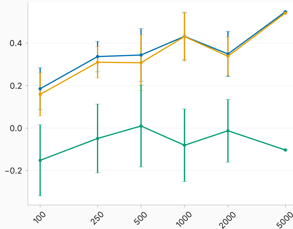
sycophancy — system prompting (L26)
