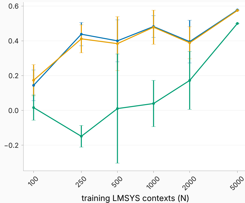
evil — many-shot (L26)
