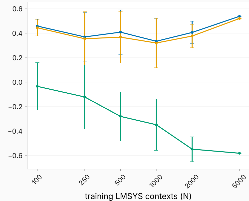
hallucination — many-shot (L27)
