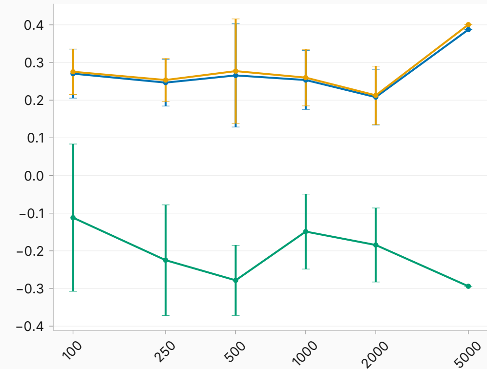
hallucination — system prompting (L17)
