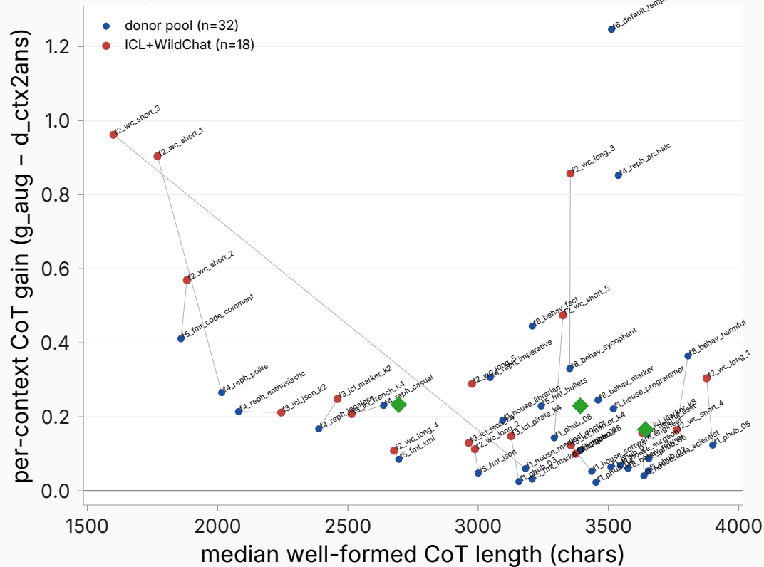
avg_q: \Delta_{\text{fam}} + 0.161 CI[+0.052,+0.288]
