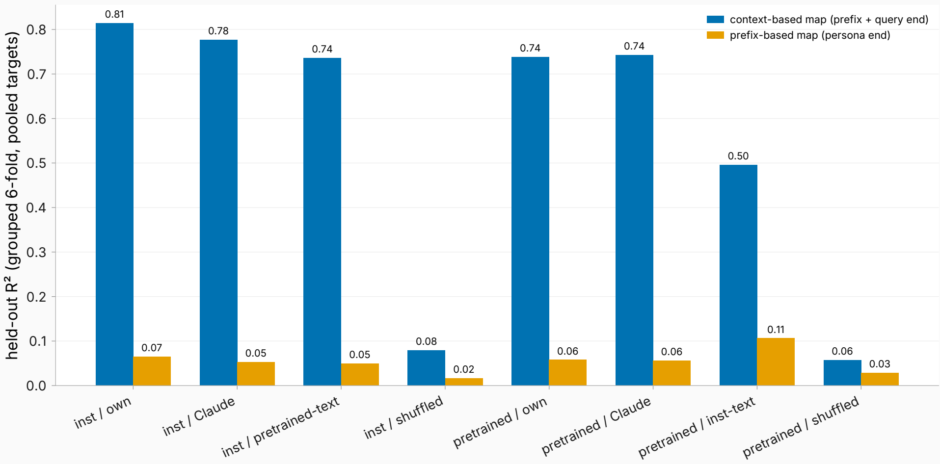
Held-out map skill per cell (layer 14, fit-arm A, ambient; battery-excluded)
