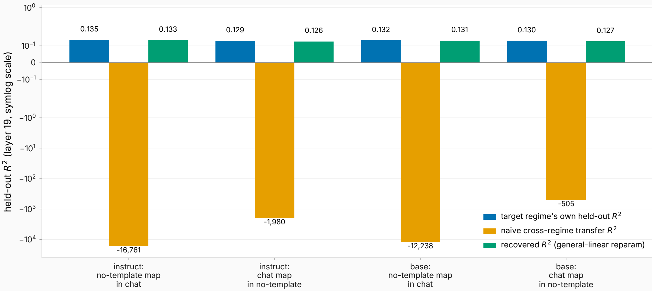
Prefix arm: naive transfer explodes; reparameterization recovers the ceiling
