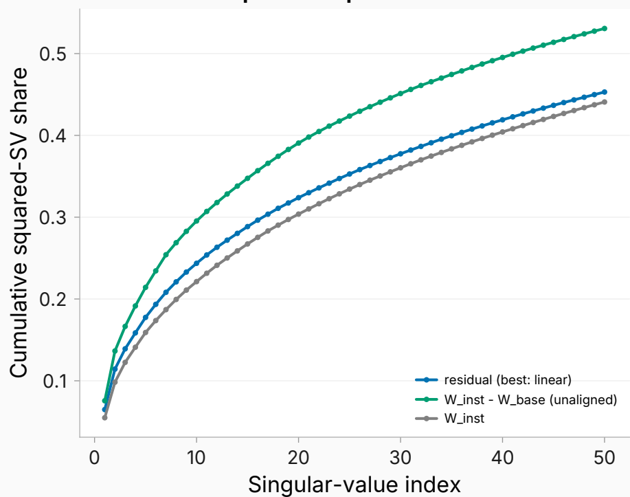
L19 residual-operator spectrum
