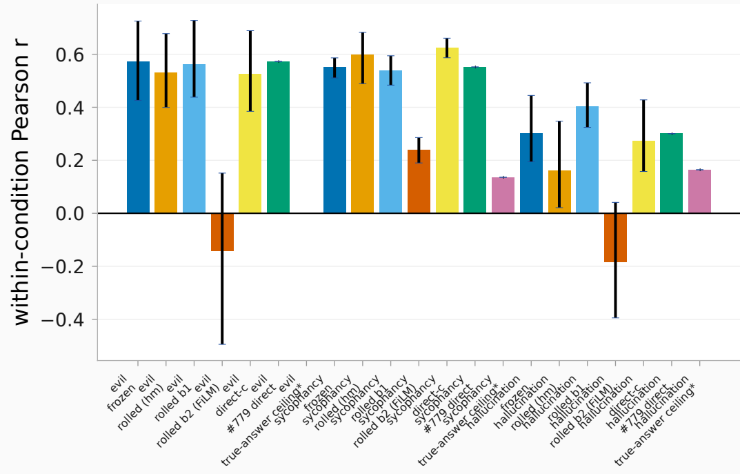
many_shot (* = captured-subset panel)
