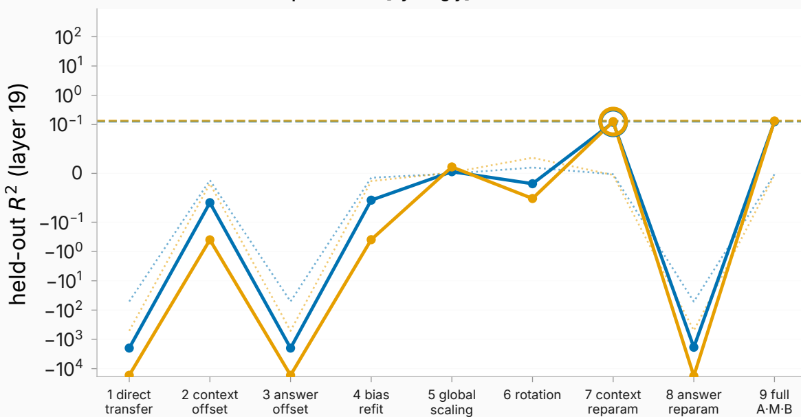
Qwen2.5-7B-Instruct — prefix arm [symlog y]
