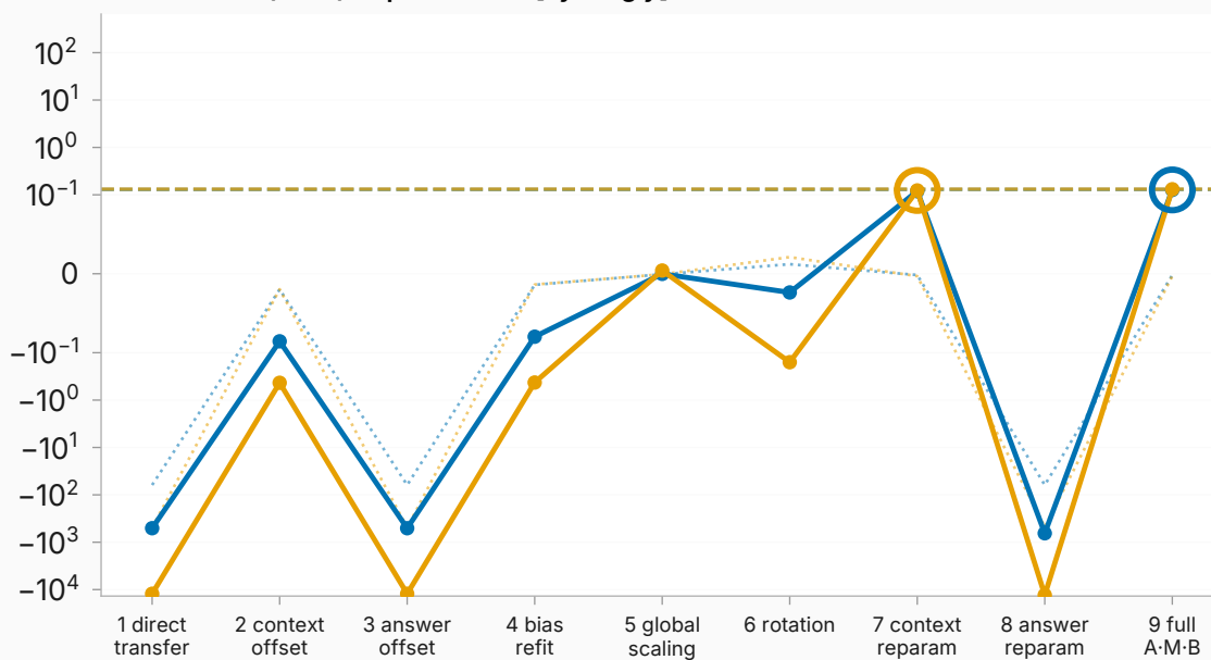
Qwen2.5-7B (base) — prefix arm [symlog y]
