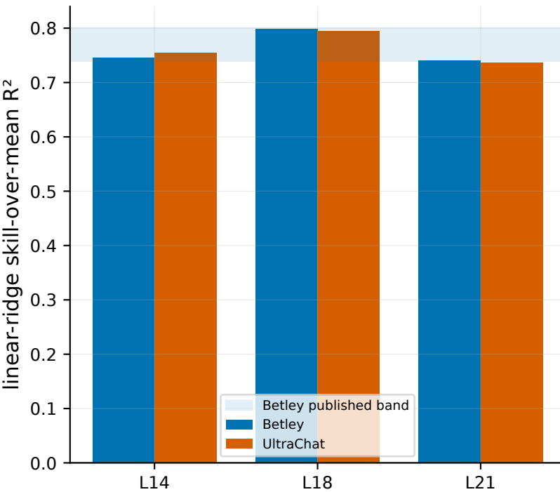
D1: c_C→v0 ridge skill (plateau)
