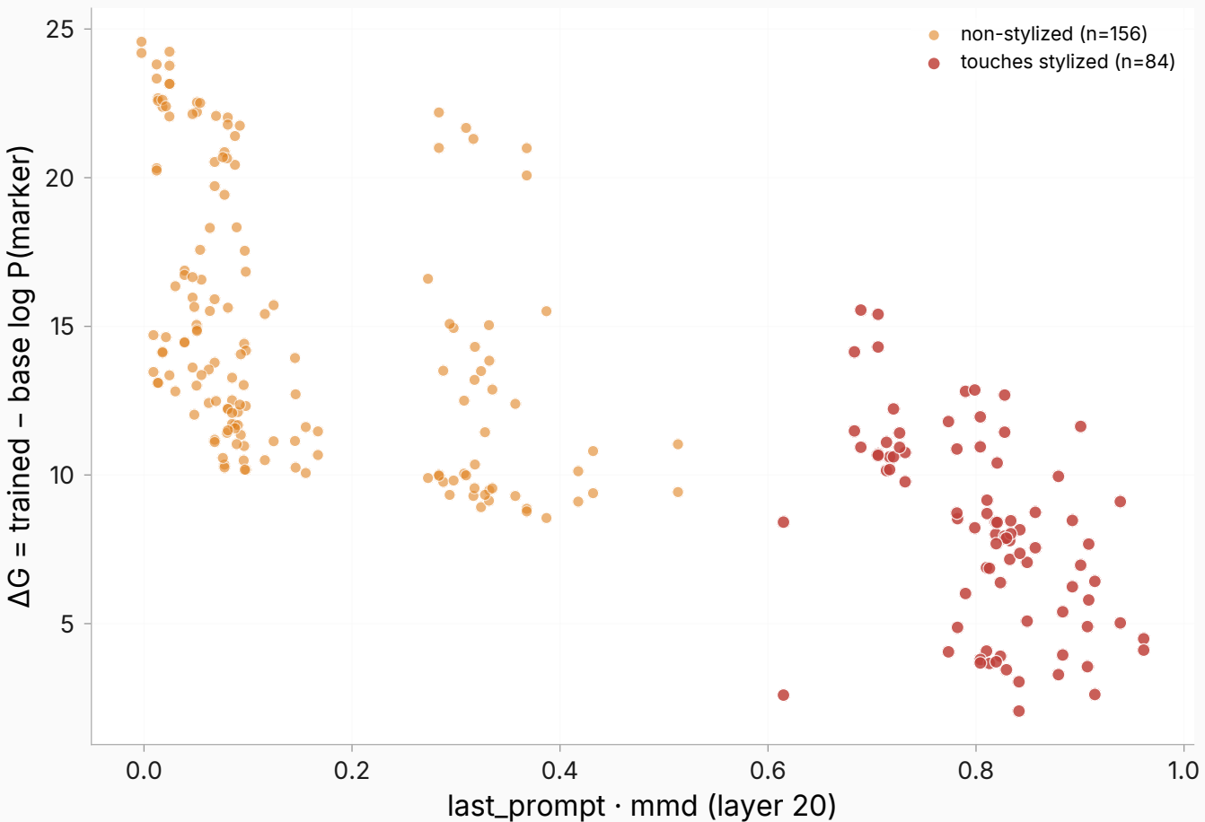
Winner: last_prompt/mmd/L20 — CV R^2=0.60
