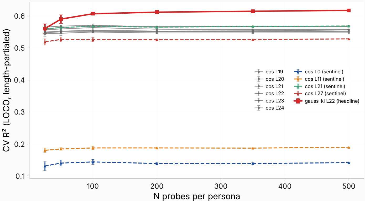
Mean-based baselines vs cloud-aware headline · loc_ep1
