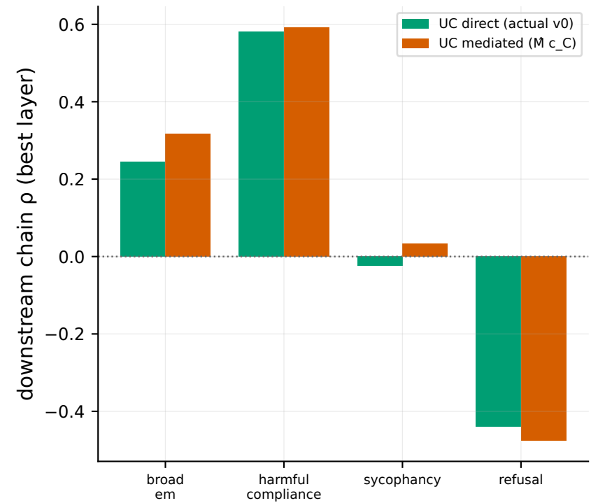
D3: behavior-chain preservation (UltraChat)
