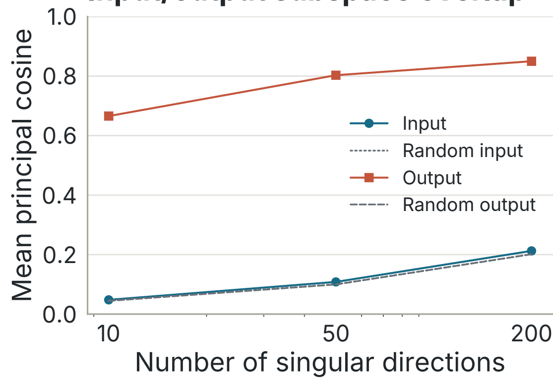
D · OPENTHINKER3-7B
