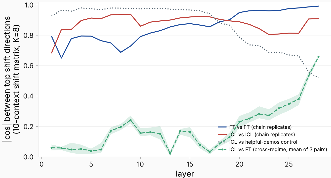
The two routes write reliably different directions (within-regime replicates \approx 0.8\text{--}0.99 ; cross-regime \approx 0.1\text{--}0.35 except the final layer)
