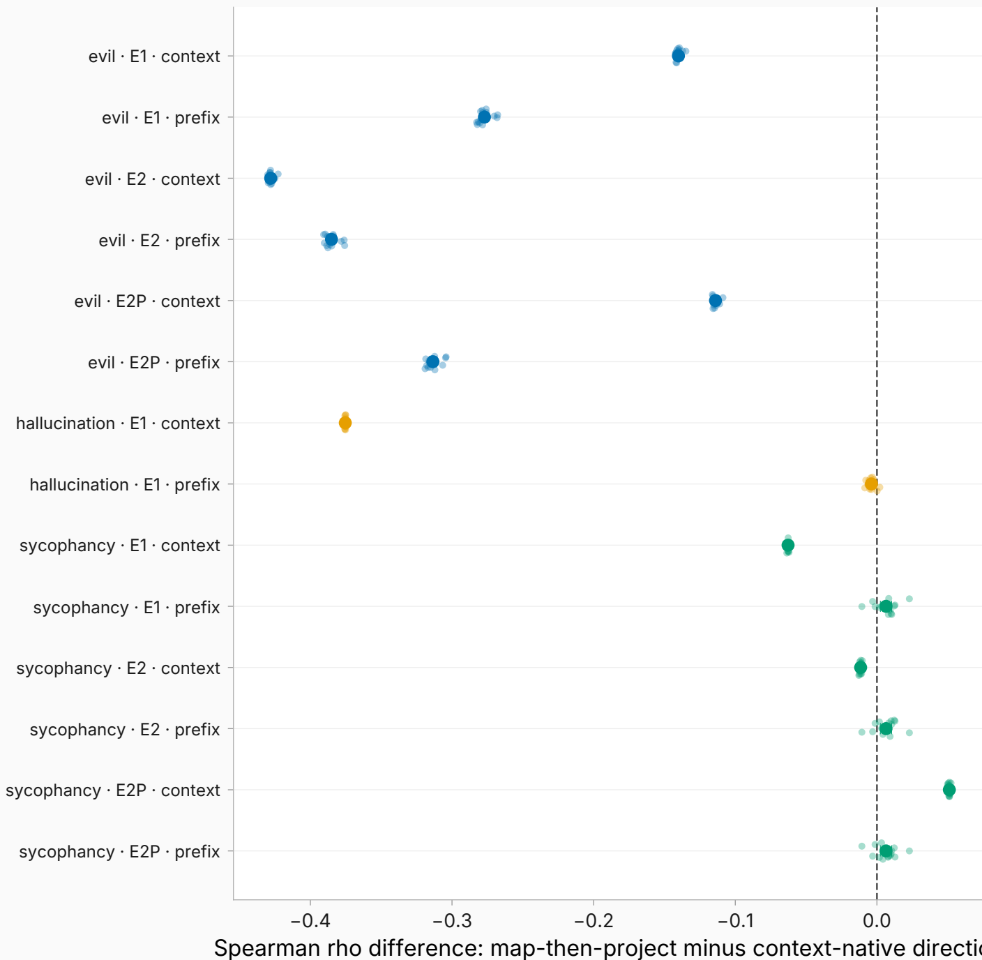
Map-then-project vs context-side projection (largest budgets; dots = per-cell values, n=15 each)
