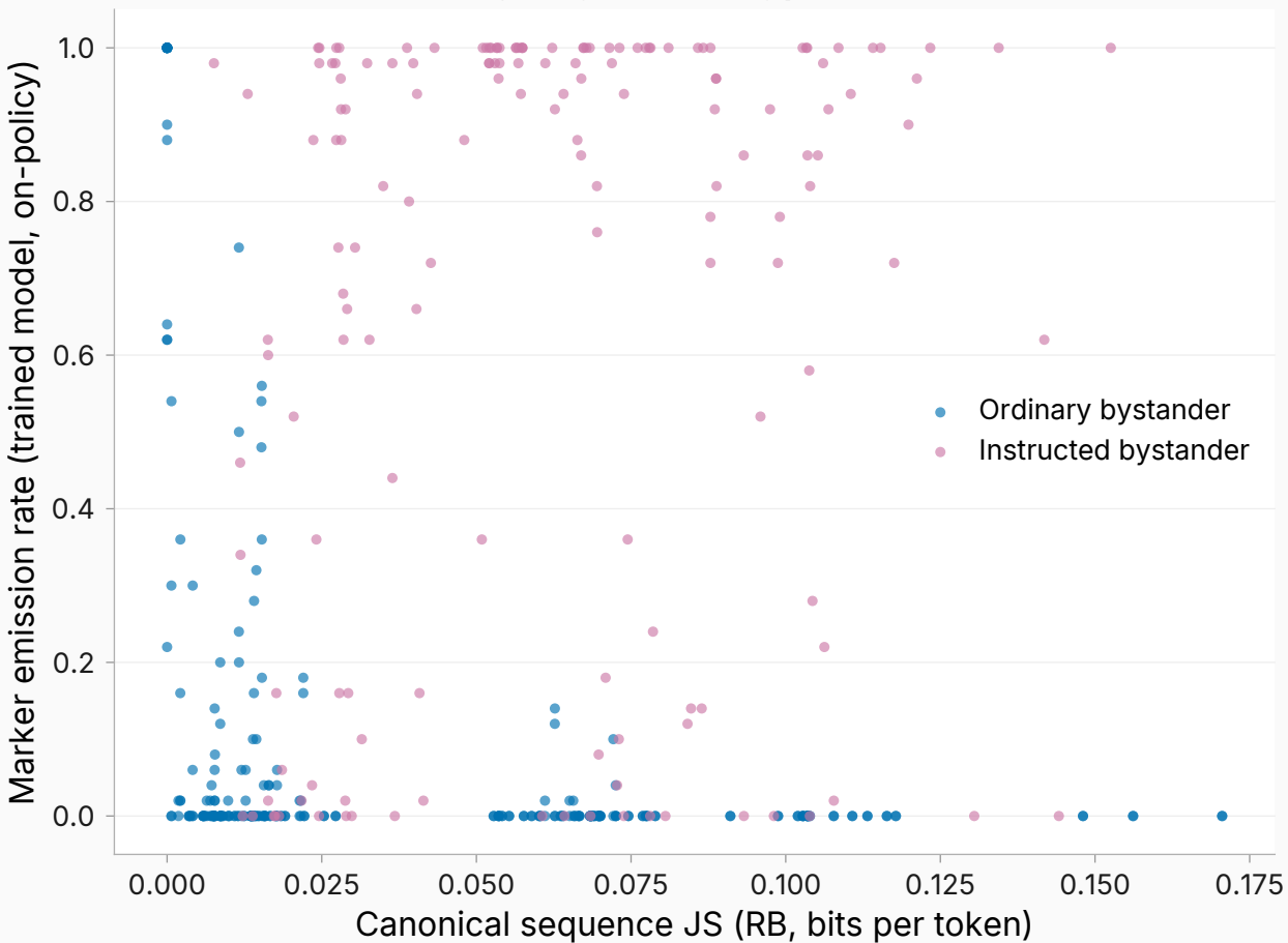
Canonical JS vs leakage, by context type
