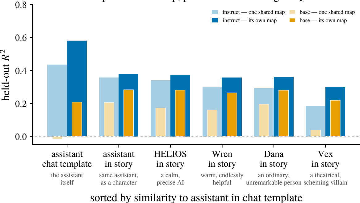
One shared map vs its own map, per character/framing — Qwen-2.5-7B
