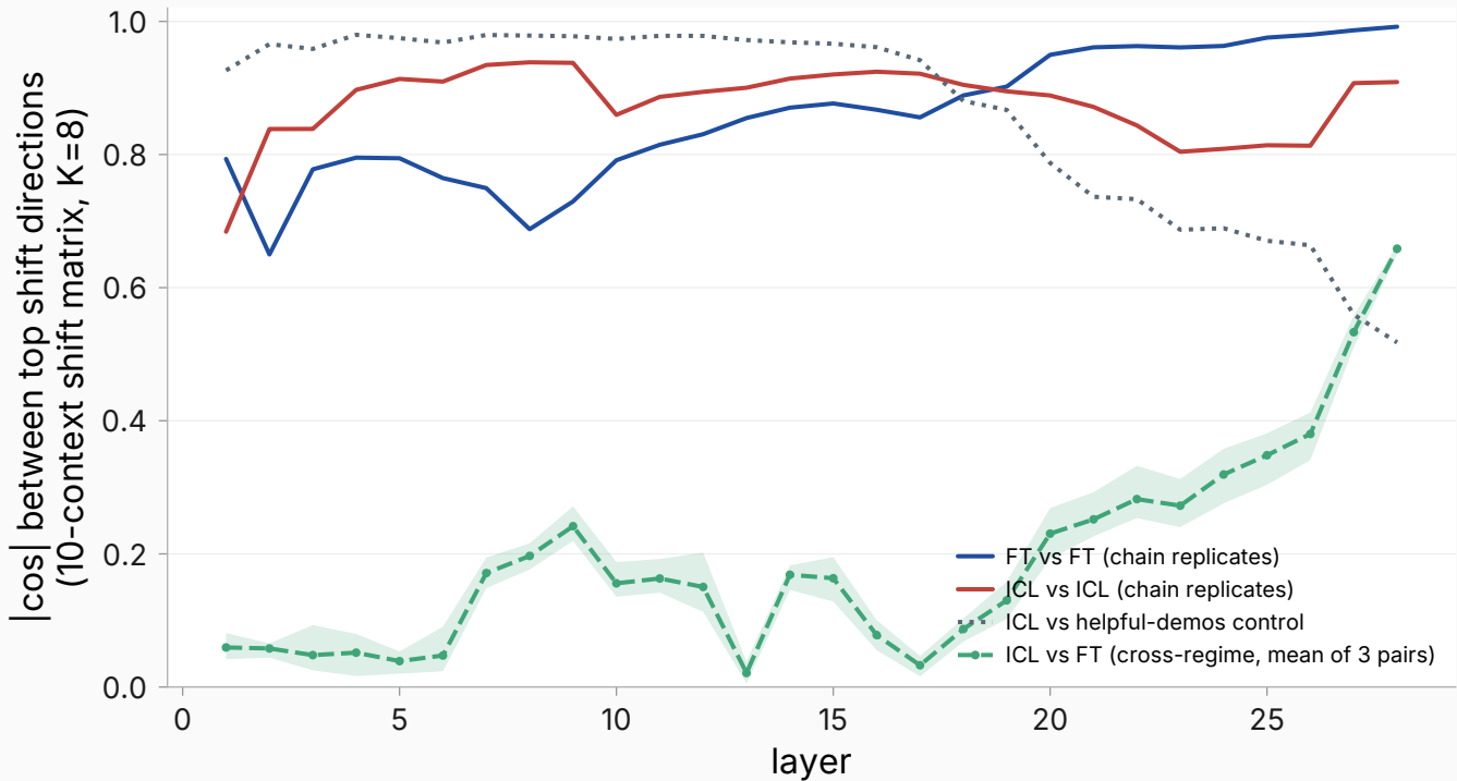
The two routes write reliably different directions (within-regime replicates 0.65–0.99; cross-regime \approx 0.1 –0.35 until the final layer)
