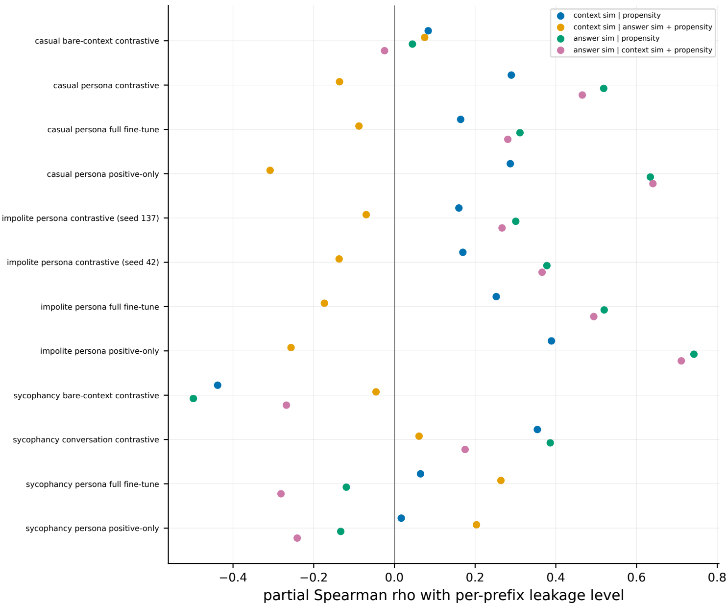
context vs answer similarity partials, base propensity always conditioned
